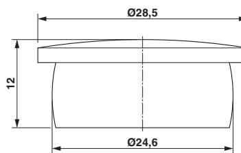
Dimensioned drawing
