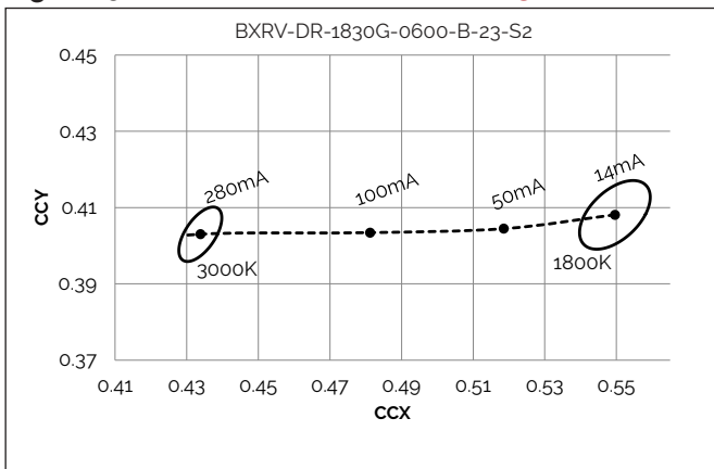
Figure 15: Color shift vs. Forward Current 3000K - 1800K
