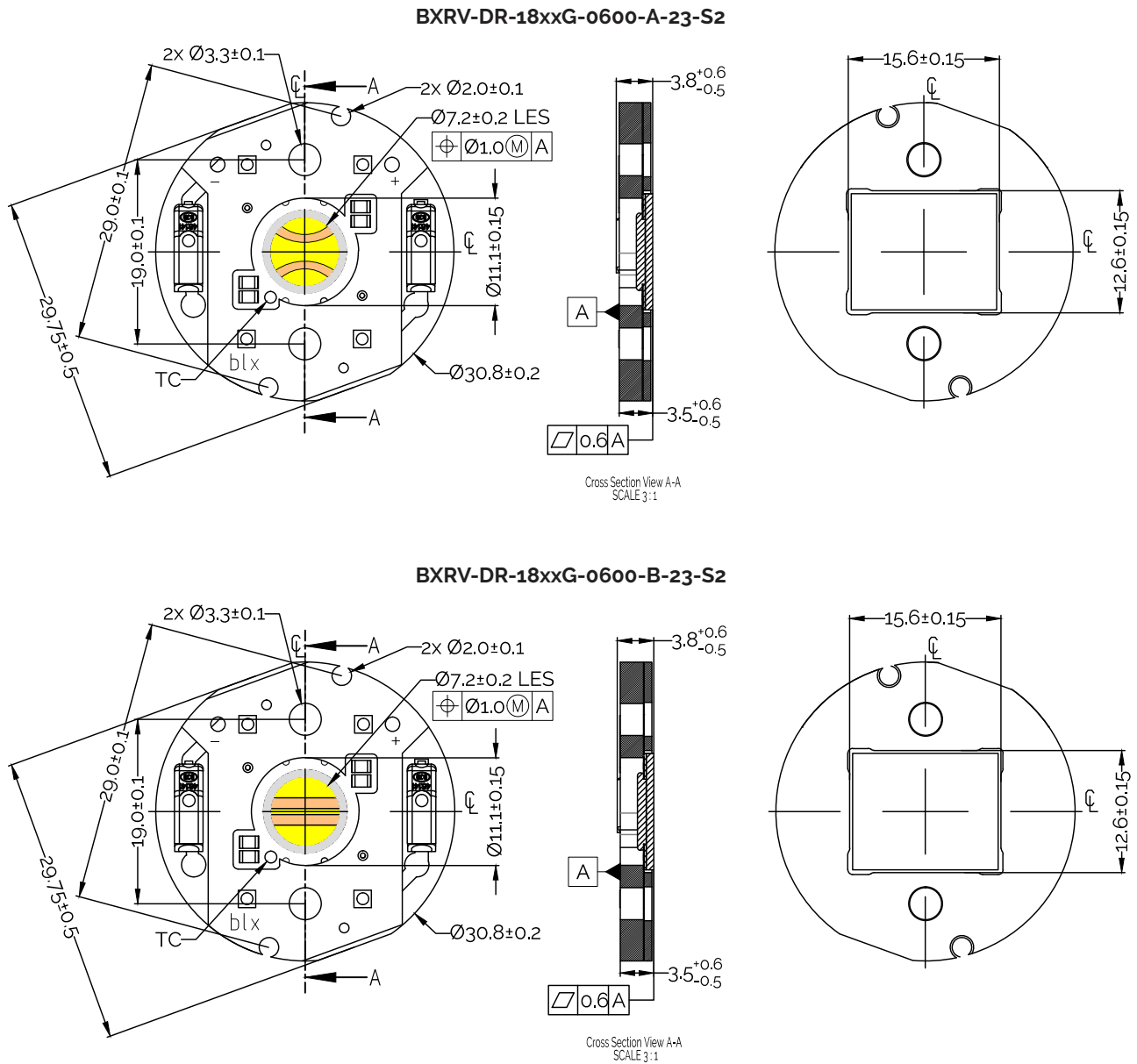
Figure 20: Mechanical Drawing Specifications
