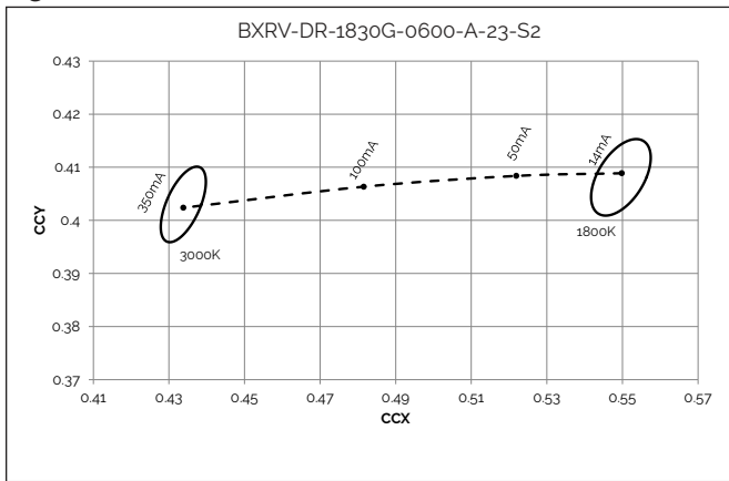
Figure 13: Color shift vs. Forward Current 3000K - 1800K
