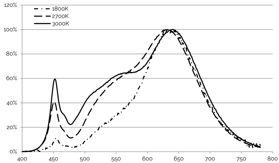
Figure 19: Typical Color Spectrum
