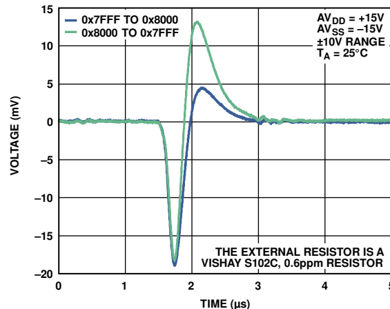
Figure 26. Digital-to-Analog Glitch
