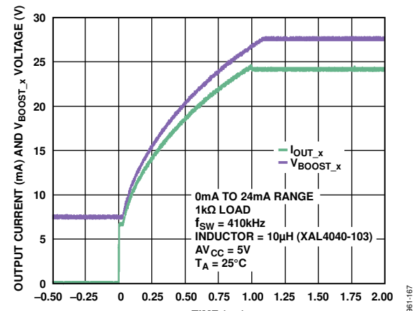
Figure 48. Output Current and V_{BOOST\_x} Settling Time with DC-to-DC Converter (See Figure 78)
