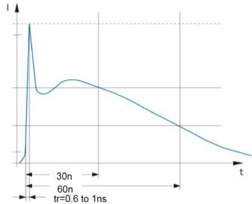
IEC61000-4-2 Waveform
