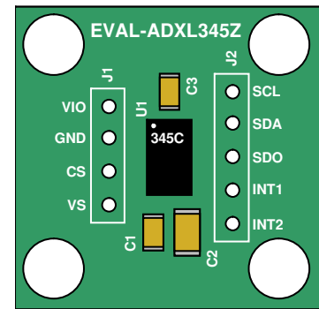
Figure 2. Physical Layout
