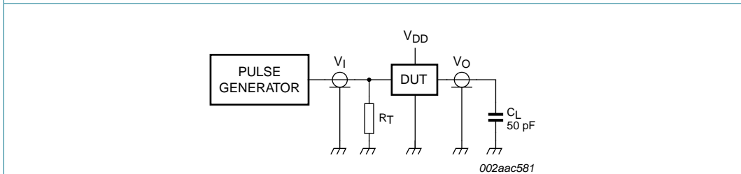
Fig 17. Test circuitry for enable/disable times, SDOUT ( t_{en(\text{SDOUT})} and t_{dis(\text{SDOUT})} )
