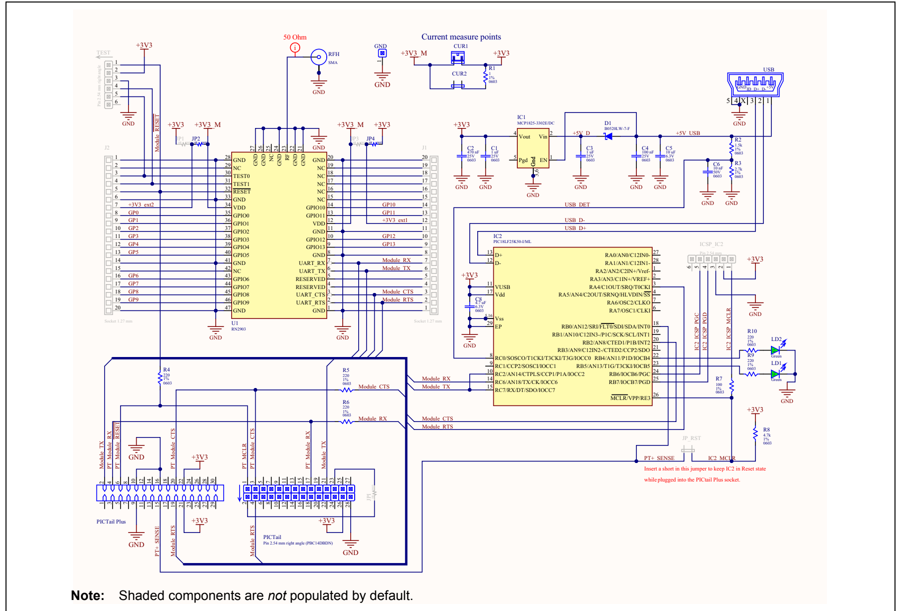
FIGURE A-1: RN2903 LoRa™ TECHNOLOGY PICtail™/PICtail PLUS DAUGHTER BOARD SCHEMATIC
