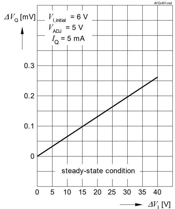
Line regulation \Delta V_{Q,line} vs. input voltage change \Delta V_I
