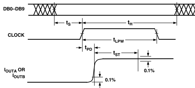
Figure 1. Timing Diagram
