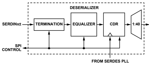
Figure 144. Deserializer Block Diagram
