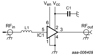
Figure 34. Schematics GNSS LNA and LTE B32 evaluation board
