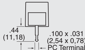
2 – Turret Type Solder Terminal
