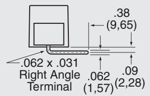
7 – Right Angle Printed Circuit Pin
