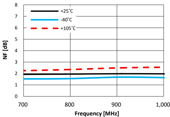
Figure 36. Noise Figure vs. Frequency @ VDD = 5V Over Temperature (Max Gain State)
