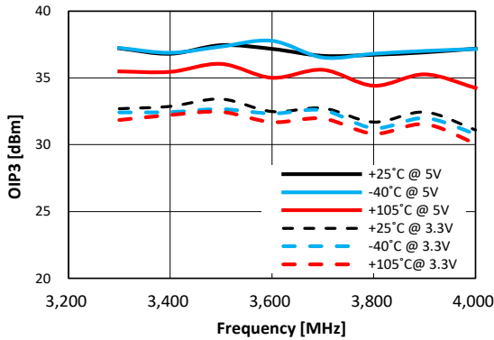
Figure 69. OIP3 vs. Frequency vs. VDD Over Temperature (Max Gain State)
