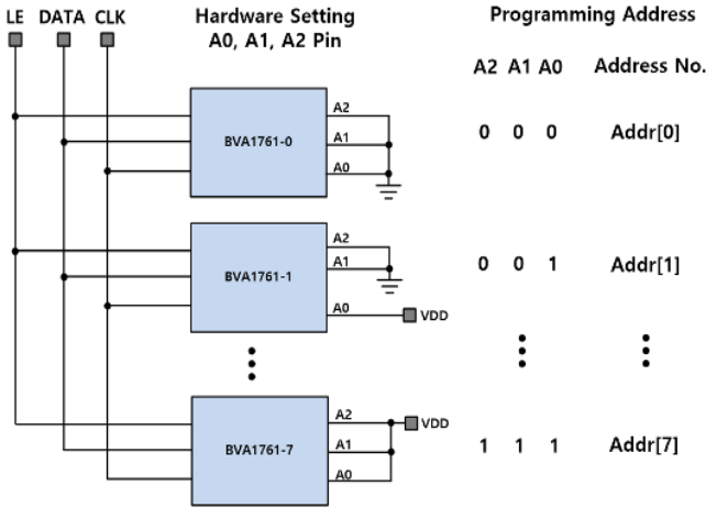
Figure 5. Multi Device Addressing Scheme using SPI
