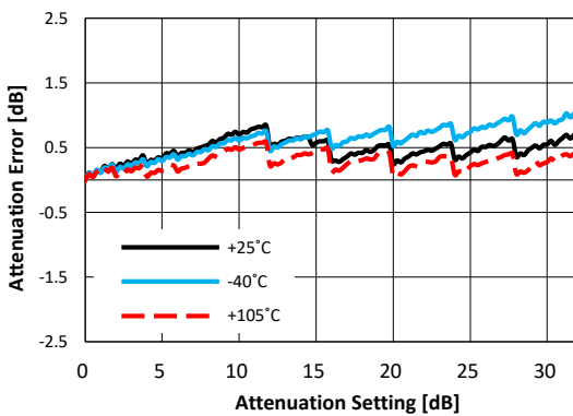
Figure 110. Attenuation Error at 5.5GHz vs Temperature Over All Attenuation States
