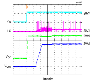
MAXM17634/MAXM17635 STARTUP THROUGH IN V_{OUT} = 5V , f_{SW} = 1MHz , 20mA LOAD, PFM MODE
