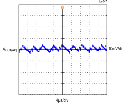
MAXM17634/MAXM17635 STEADY-STATE OUTPUT-VOLTAGE RIPPLE V_{OUT} = 5V , f_{SW} = 1MHz , 20mA LOAD, DCM MODE
