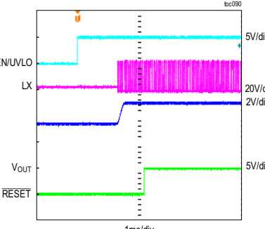
MAXM17634/MAXM17635 STARTUP THROUGH ENABLE (3.3V PREBIAS) V_{OUT} = 5V , f_{SW} = 1MHz , FULL LOAD, PWM MODE
