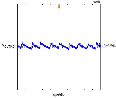
MAXM17633/MAXM17635 STEADY-STATE OUTPUT-VOLTAGE RIPPLE V_{OUT} = 3.3V , f_{SW} = 800kHz , 20mA LOAD, DCM MODE
