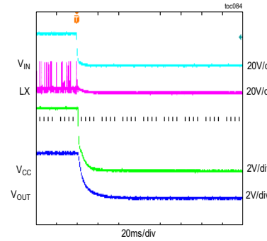
MAXM17633/MAXM17635 SHUTDOWN THROUGH IN V_{OUT} = 3.3V , f_{SW} = 800kHz , 20mA LOAD, PFM MODE
