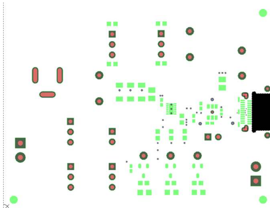
Figure 13. Top Solder Mask
