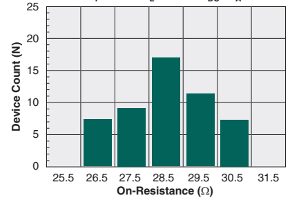
Typical On-Resistance Distribution (N=50, I_F=5\text{mA} , I_L=100\text{mA}_{DC} , T_A=25^\circ\text{C} )
