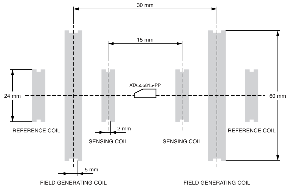
Figure 9-3. Testing Geometry
