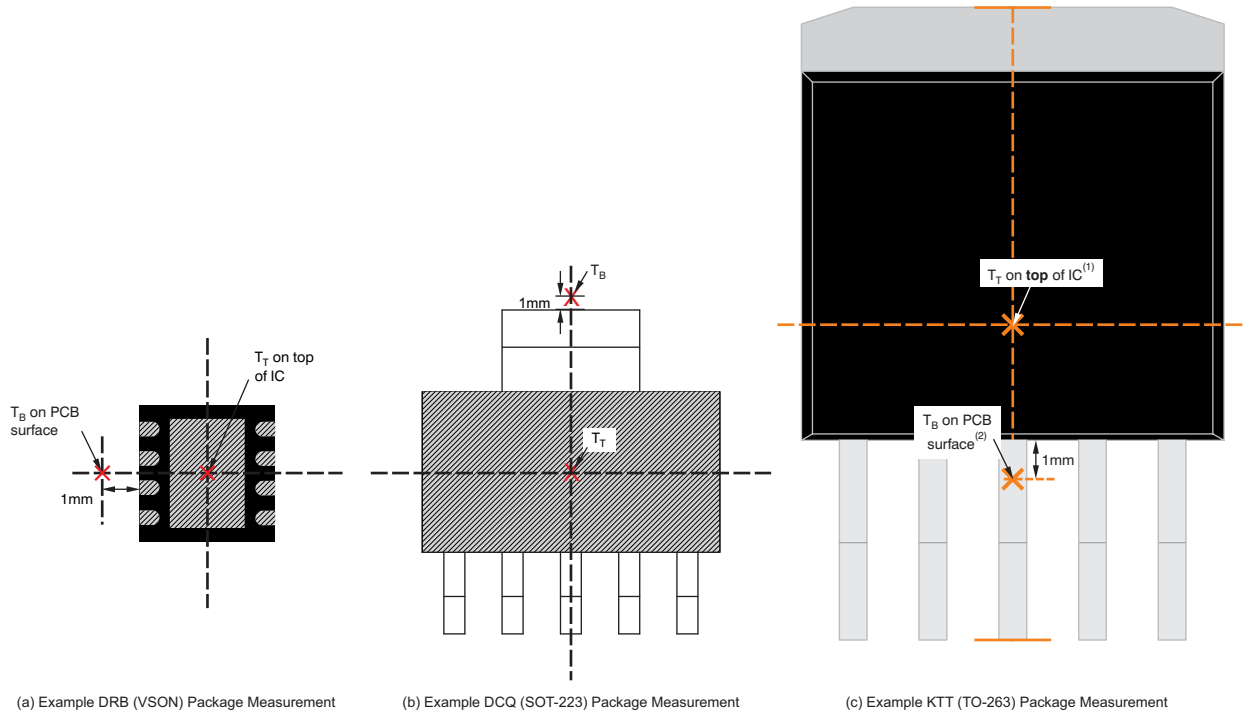
(a) Example DRB (VSON) Package Measurement (b) Example DCQ (SOT-223) Package Measurement (c) Example KTT (TO-263) Package Measurement
