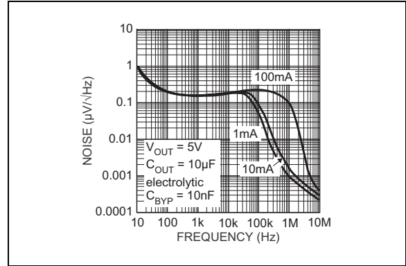
FIGURE 2-18: Noise Performance.
