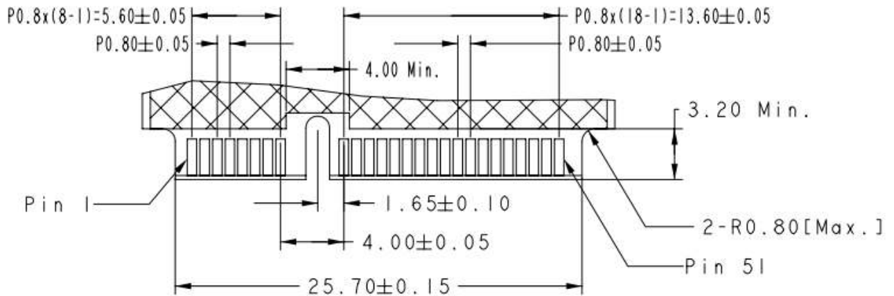
Figure 1-1 Pin Assignment
