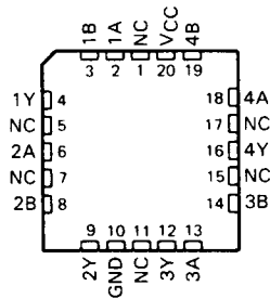
SN54HC36 . . . FK PACKAGE (TOP VIEW)
