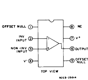
1e.—CA741C and CA741E with internal phase compensation.
