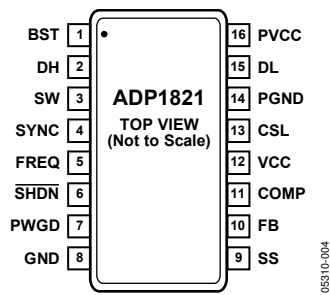
Figure 4. Pin Configuration
