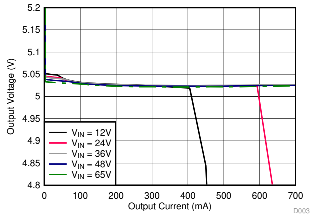
Figure 23. Load Regulation (Linear Scale)
