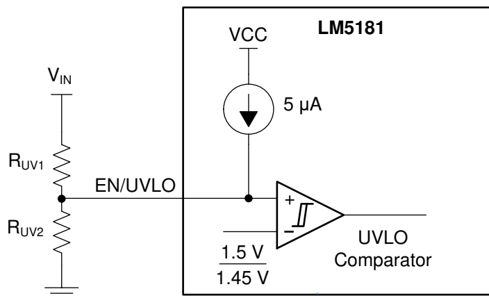
Figure 19. Programmable Input Voltage UVLO With Hysteresis
