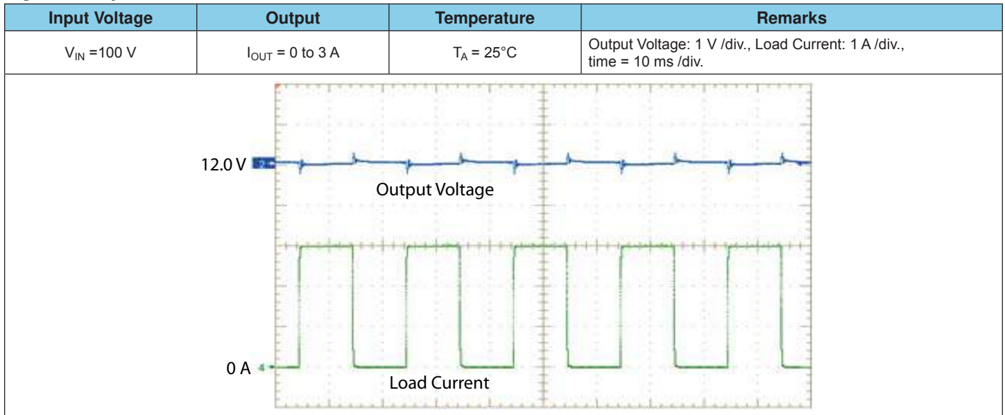
Figure 20. Dynamic Load
