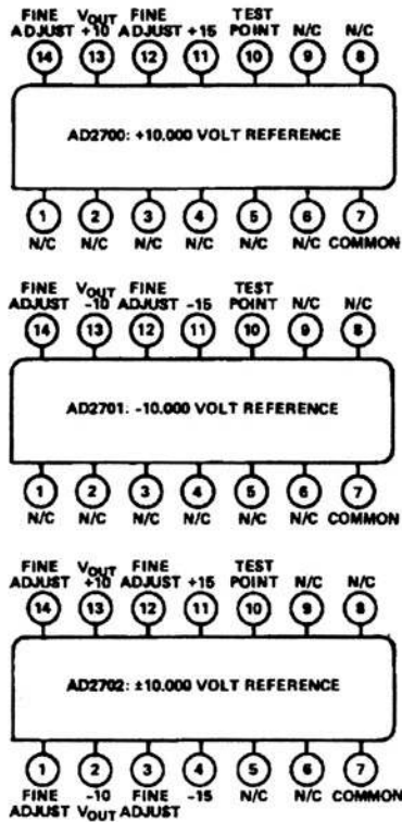
Pin Designations
