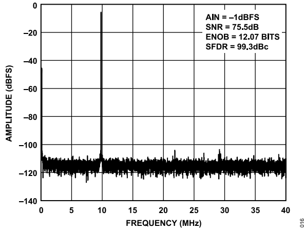
Figure 10. Single-Tone 16k FFT with f_{IN} = 9.7 \text{ MHz} , f_{SAMPLE} = 80 \text{ MSPS}
