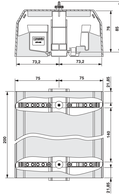
Dimensioned drawing
