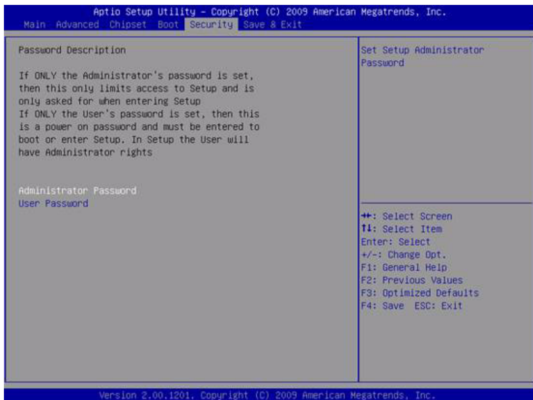
Figure 3.18 Security Configuration
