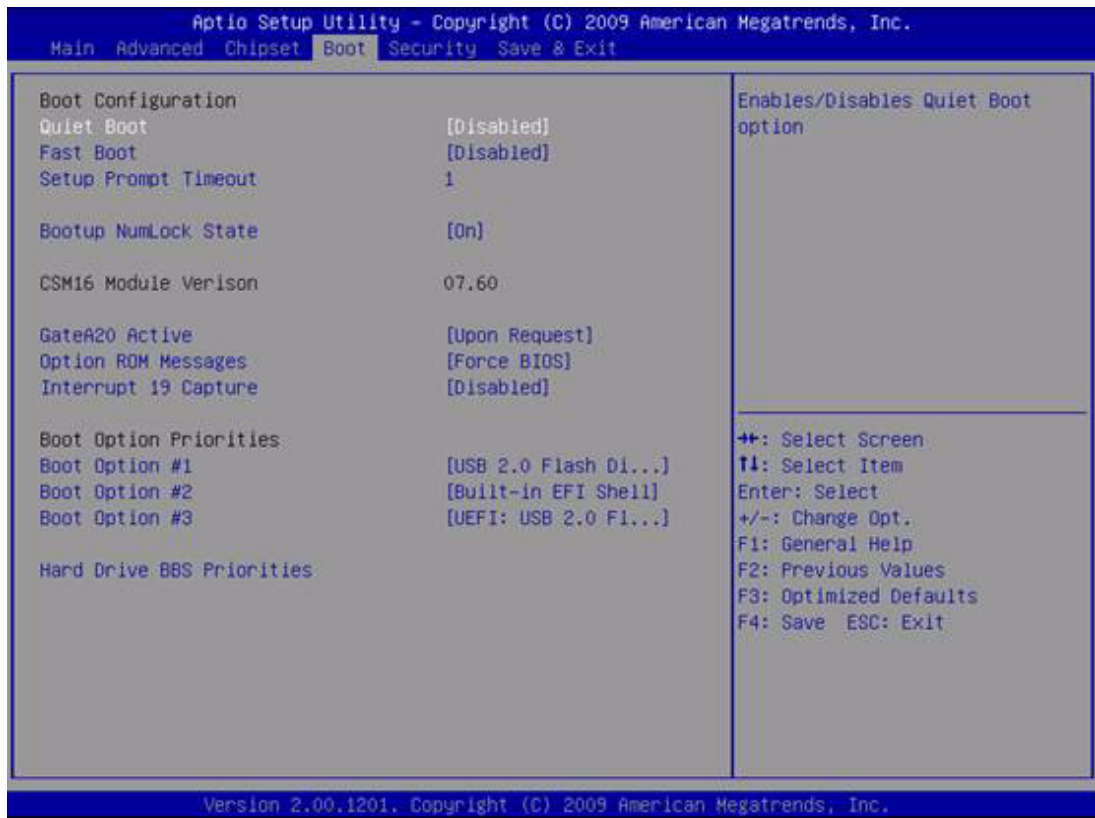
Figure 3.17 Boot Configuration
