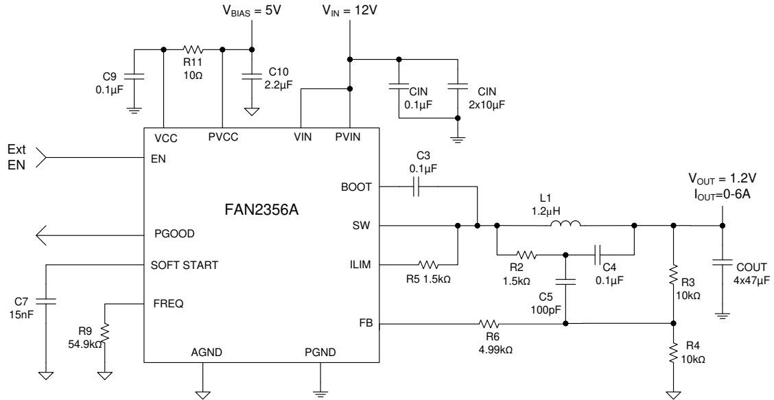
Figure 1. Typical Application
