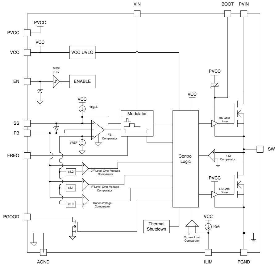
Figure 2. Block Diagram
