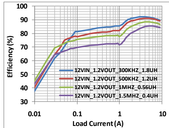
Figure 8. Efficiency vs. Load Current with V_{IN}=12\text{ V} and V_{OUT}=1.2\text{ V}
