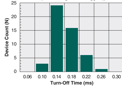
Typical Turn-Off Time (N=50, I_F=2\text{mA} , I_L=120\text{mA}_{\text{DC}} , T_A=25^\circ\text{C} )
