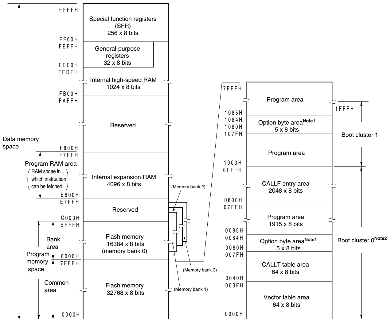
Figure 3-6. Memory Map ( \mu PD78F0536)
