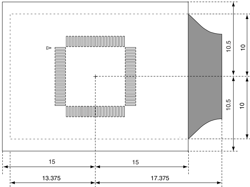
Figure B-1. For 64-Pin GB Package
