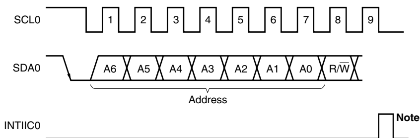
Figure 17-14. Address
