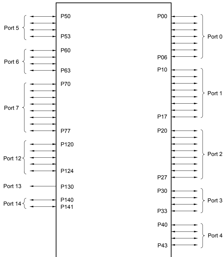
Figure 5-1. Port Types
