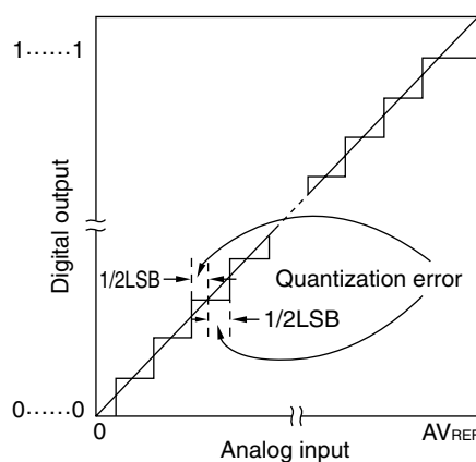
Figure 13-15. Quantization Error
