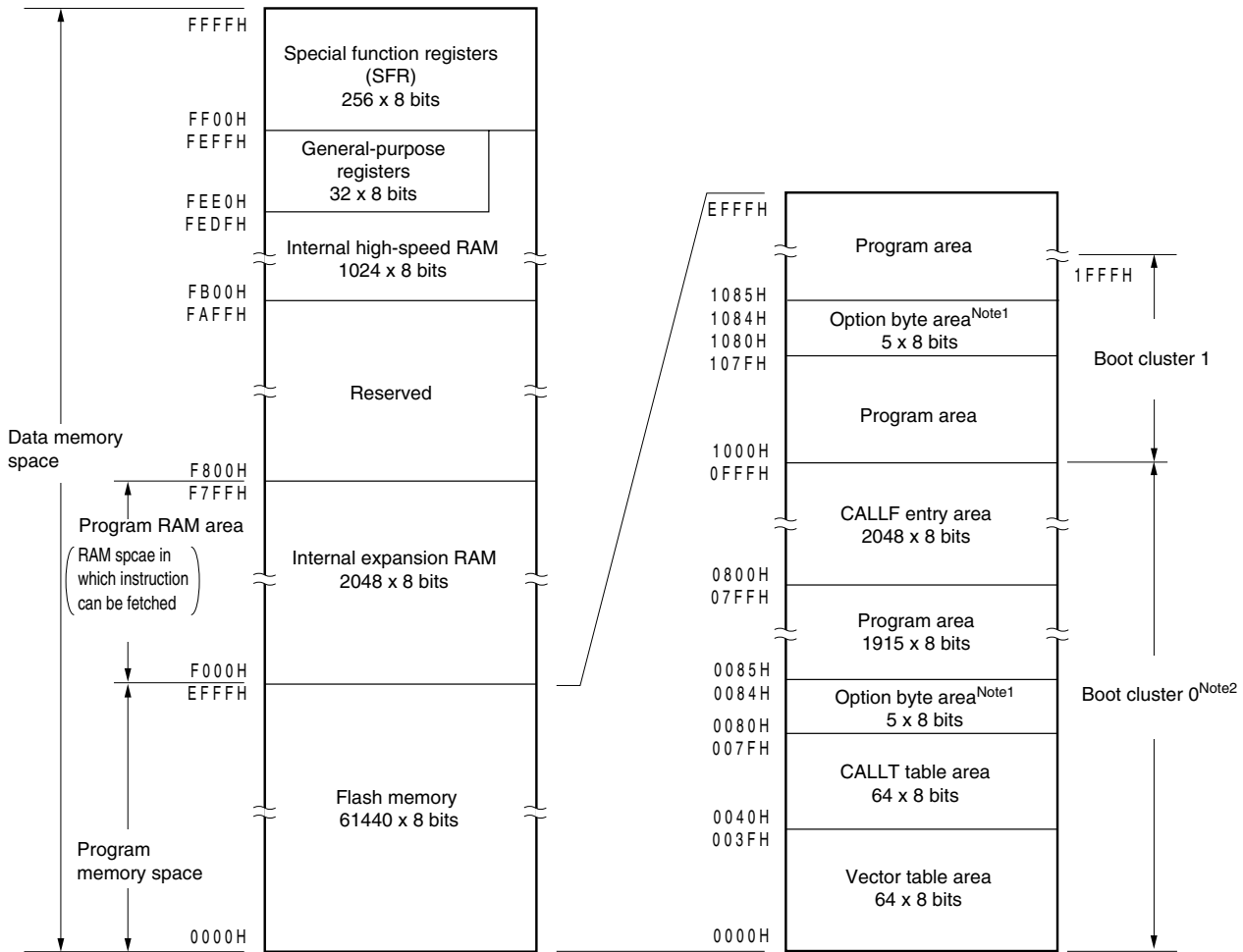
Figure 3-5. Memory Map ( \mu PD78F0535)
