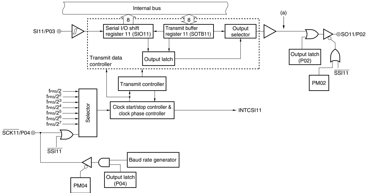
Figure 16-2. Block Diagram of Serial Interface CSI11 (Available only in the \mu PD78F0534, 78F0535, 78F0536, 78F0537, 78F0537D)
