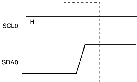
Figure 17-17. Stop Condition
