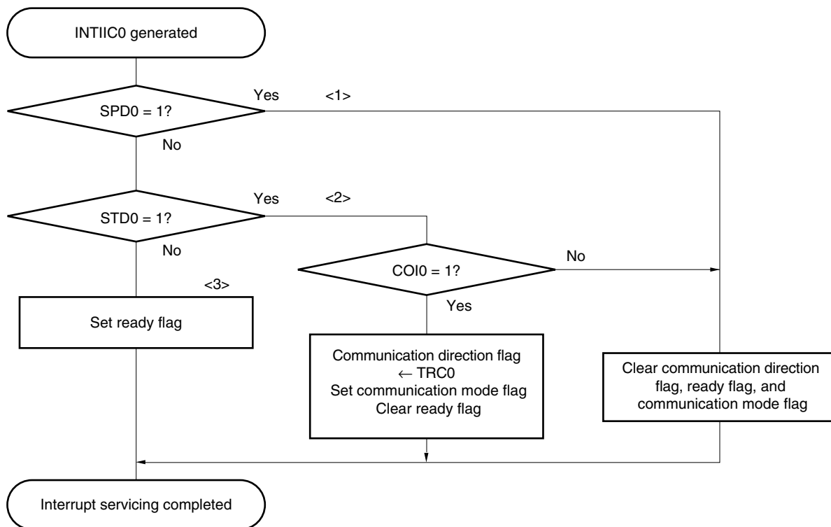
Figure 17-26. Slave Operation Flowchart (2)
