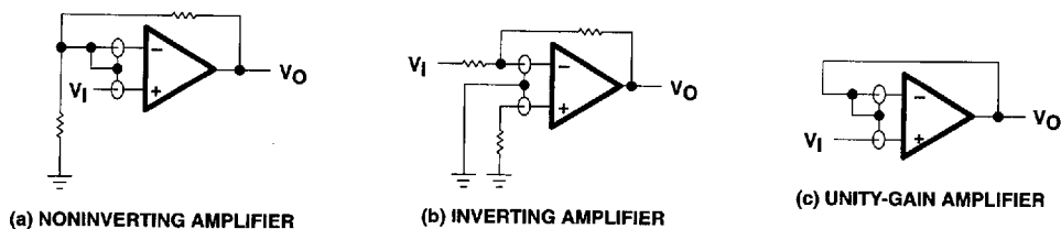
Figure 40. Guard-Ring Schemes
