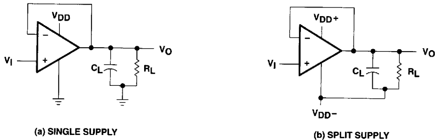
Figure 1. Unity-Gain Amplifier
