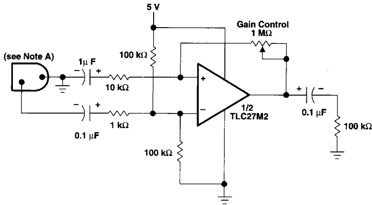
Figure 46. Microphone Preamplifier
