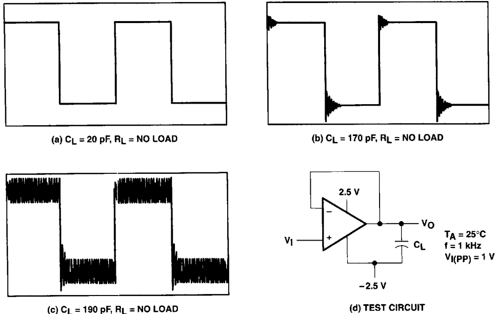
Figure 41. Effect of Capacitive Loads and Test Circuit
