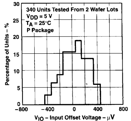
DISTRIBUTION OF TLC27M7 INPUT OFFSET VOLTAGE
