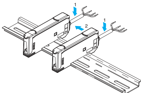
Sensor head connector catches
