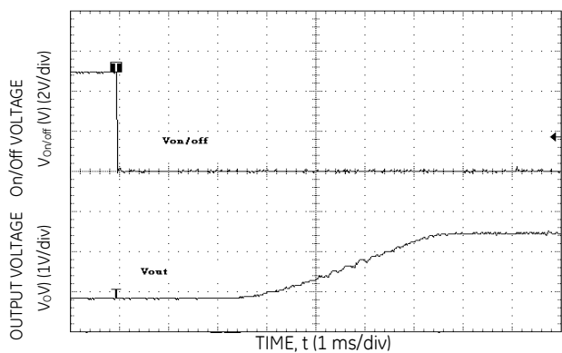
Figure 15. Typical Start-Up Using Remote On/Off with Low-ESR external capacitors ( 7 \times 150 µF Polymer) ( V_{in} = 12 Vdc, V_o = 3.3 Vdc, I_o = 6.0 A, C_o = 1050 µF).
