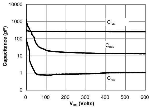
Figure 9: Capacitance Characteristics
