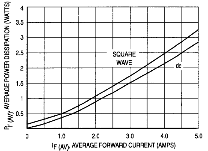
Figure 4. Power Dissipation
