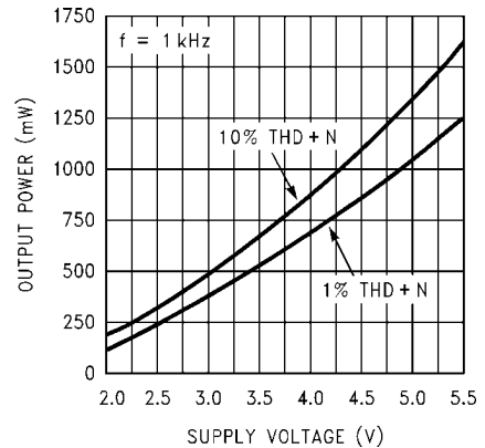
Output Power vs Supply Voltage, 8\Omega
