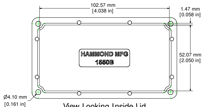
View Looking Inside Lid
