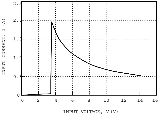
Figure 1. MH005-Series Typical Input Characteristics with I_o = I_{o, max} and T_A = 25\text{ }^\circ\text{C}
