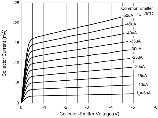
Fig. 5 - Static Characteristics
