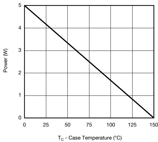
Power, Junction-to-Foot
