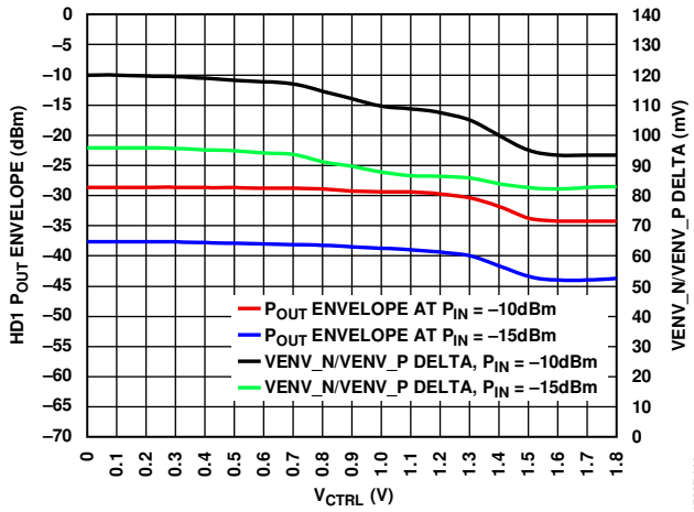
Figure 66. HD1 P_{OUT} Envelope and V_{ENV\_N}/V_{ENV\_P} Delta vs. V_{CTRL} at Various Total Input Power ( P_{IN} ) Levels, Measurements Performed at 28 GHz with Two Input Tones with Separation of 100 MHz
