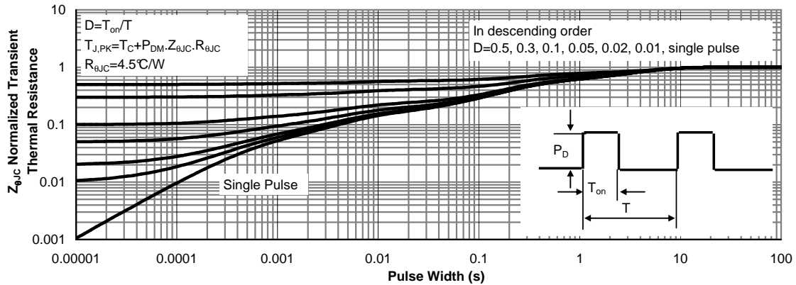
Figure 14: Normalized Maximum Transient Thermal Impedance for AOWF10T60 (Note F)
