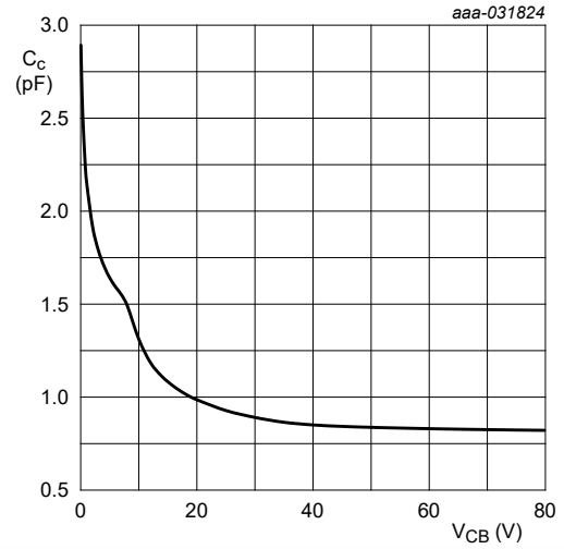
Fig. 20. NHUMD13, TR1 (NPN): Collector capacitance as a function of collector-base voltage; typical values
