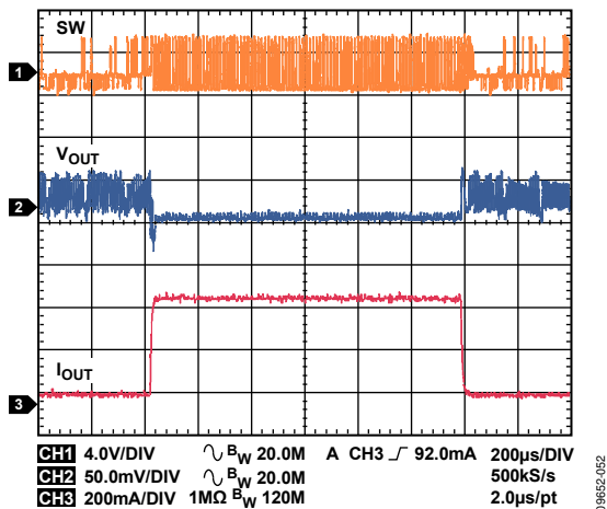
Figure 52. Buck Response to Load Transient, I_{OUT1} = 50\text{ mA to } 500\text{ mA} , V_{OUT1} = 1.2\text{ V} , Auto Mode
