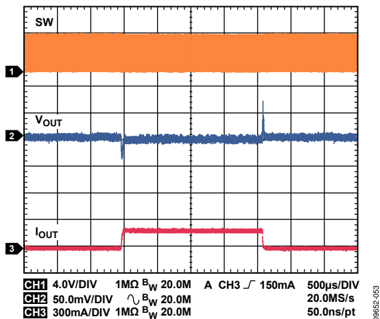
Figure 53. Buck Response to Load Transient, I_{OUT1} = 20\text{ mA to } 200\text{ mA} , V_{OUT1} = 3.3\text{ V} , PWM Mode
