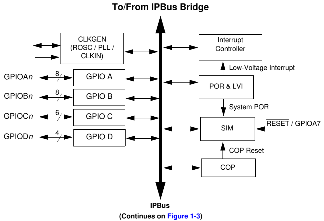
Figure 1-2 Peripheral Subsystem
