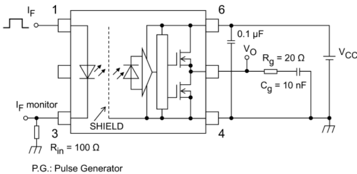
Fig. 13.1.7 Switching Time Test Circuit and Waveform
