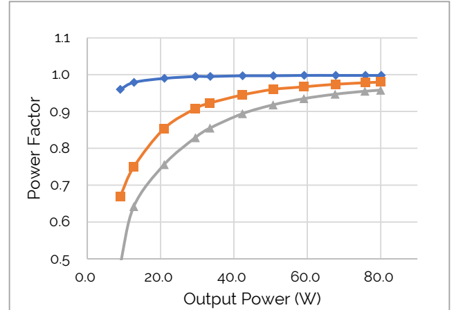
Figure 4: Power Factor vs. Output Power
