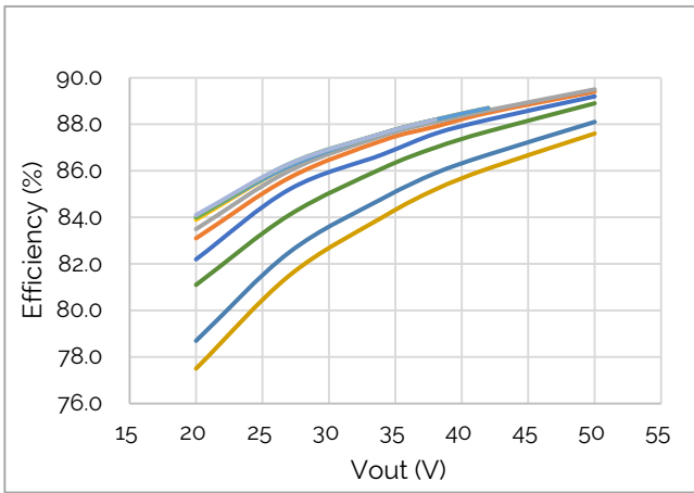
Figure 10: Efficiency @ 347VAC
