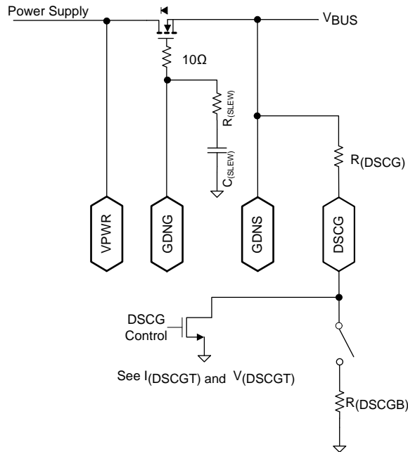
Figure 28. Discharge Schematic
